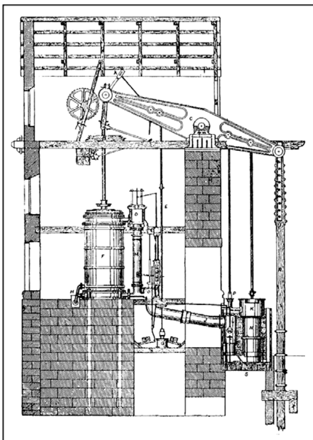
Afb. 8 The Cornish Pumping Engine. Uit: E. Henry Davies, F.G.S., Machinery for Metalliferous Mines (London 1894).
